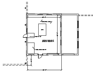
1 EXISTING PLAN - BLDG 8 SCALE: 1/16" = 1' - 0"
