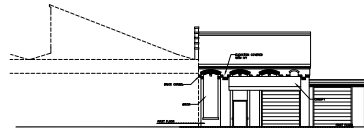
1 EXISTING ELEVATION - BLDG 8 SCALE: 1/16" = 1' - 0"
